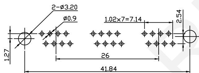
PCB Layout
