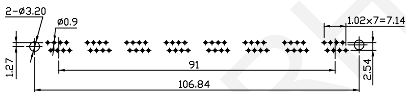
PCB Layout
