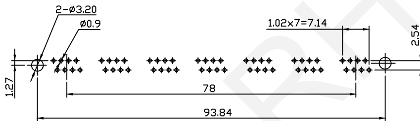
PCB Layout
